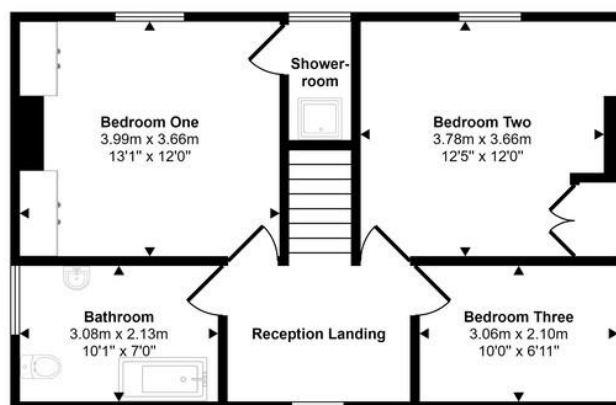
First Floor Approx 55 sq m / 591 sq ft
