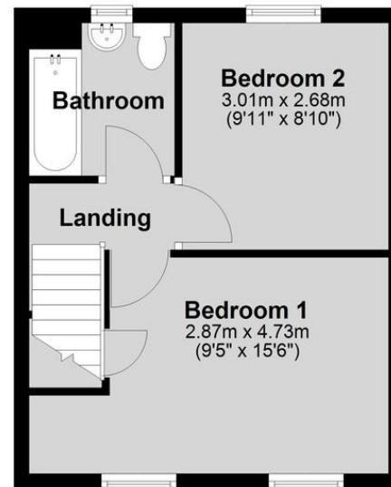
First Floor Approx. 28.4 sq. metres (305.4 sq. feet)
