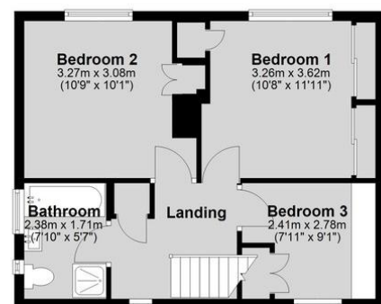
First Floor Approx. 42.2 sq. metres (454.0 sq. feet)
