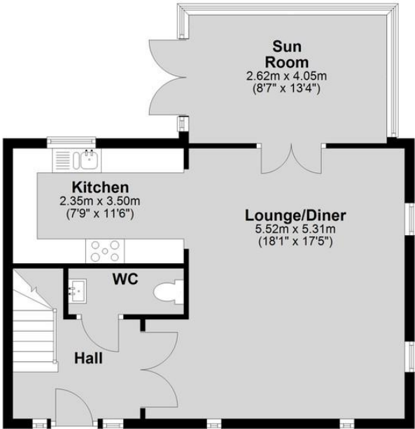
Ground Floor Approx. 56.2 sq. metres (605.2 sq. feet)
