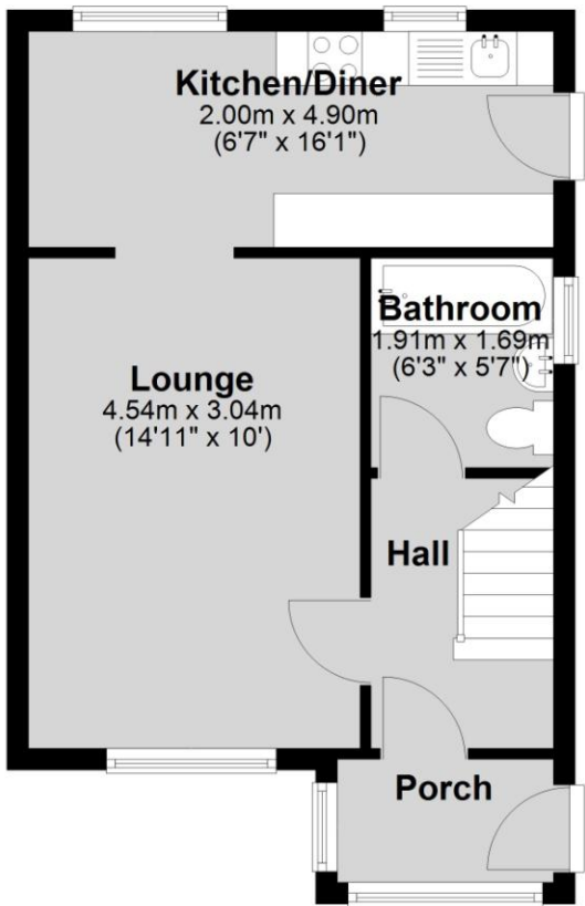
Total area: approx. 64.9 sq. metres (698.5 sq. feet)
