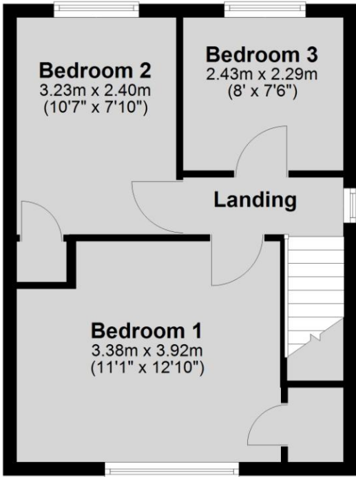
First Floor Approx. 30.2 sq. metres (325.6 sq. feet)
