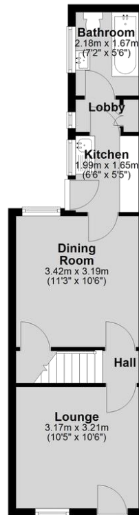
Ground Floor Approx. 33.2 sq. metres (357.9 sq. feet)
