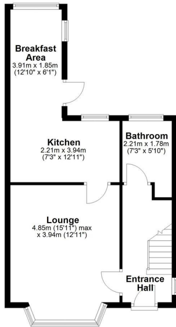
Ground Floor Approx. 46.0 sq. metres (495.2 sq. feet)
